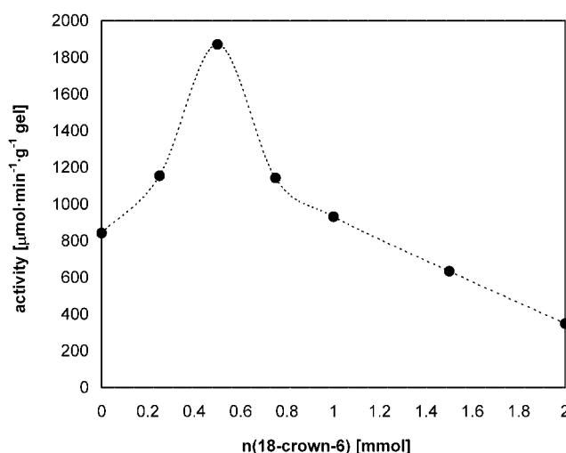
Figure 2. Influence of different amounts of 18-crown-6 as an additive (see text).
