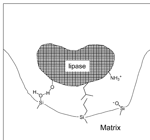
Figure 1. Schematic view of non-covalent interactions between the gel matrix and the lipase.
