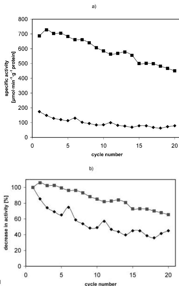
Figure 3. Recycling experiments in the kinetic resolution of rac - 6 using sol-gel CaLB-immobilizate (■) and commercial CaLB powder (◆). a) Specific activity. b) Decrease in activity (%).
