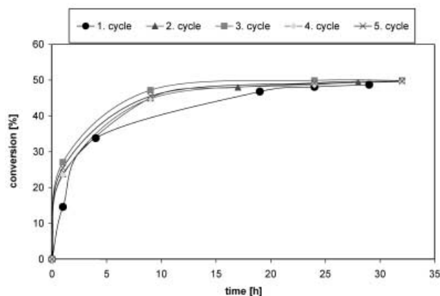
Figure 4. Recycling experiments in the kinetic resolution of rac -13 using the sol-gel CaLB-immobilizate prepared with 18-crown-6 as an additive.
